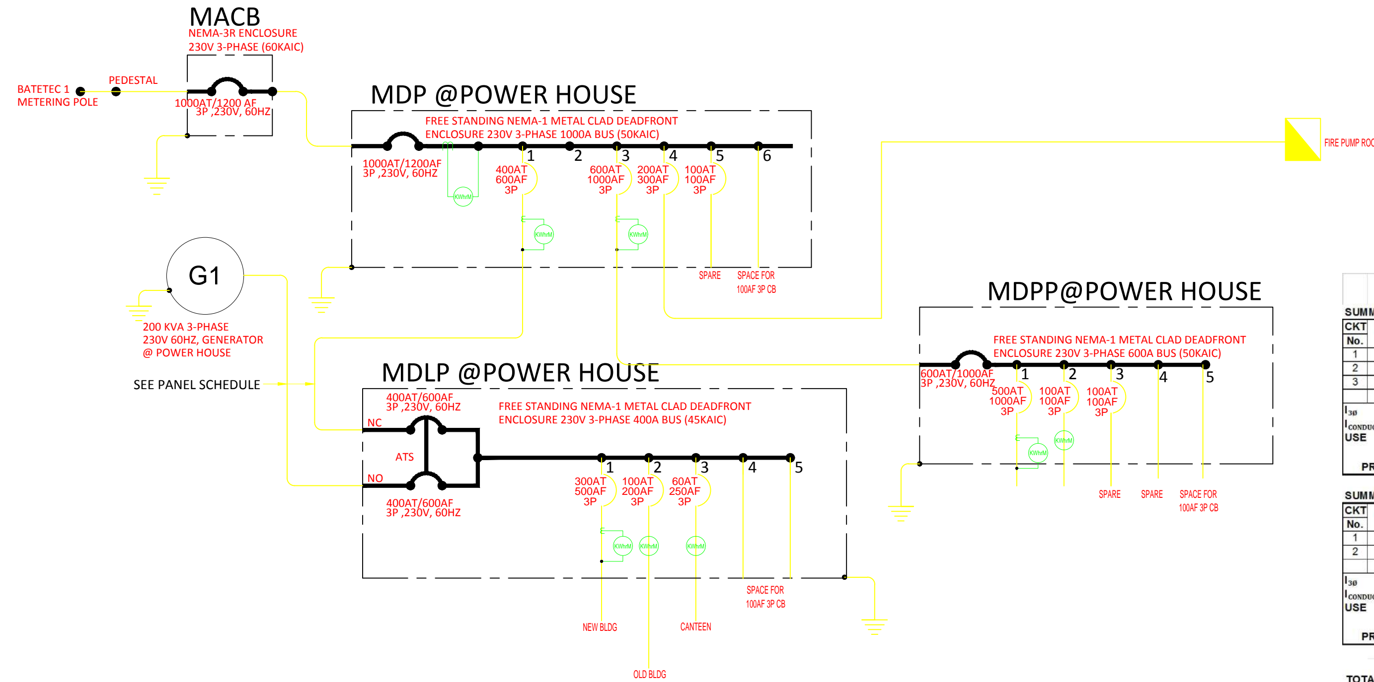
1 SINGLE LINE DIAGRAM SCALE: E-2 NTS
